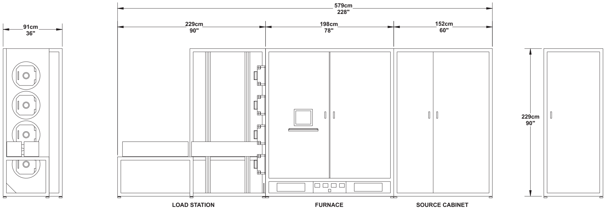
ProTemp Sirius™ PRO 200 Semiconductor Diffusion Furnace
